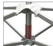
Roof Tensioning
