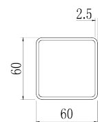
4. Roof Purlin
