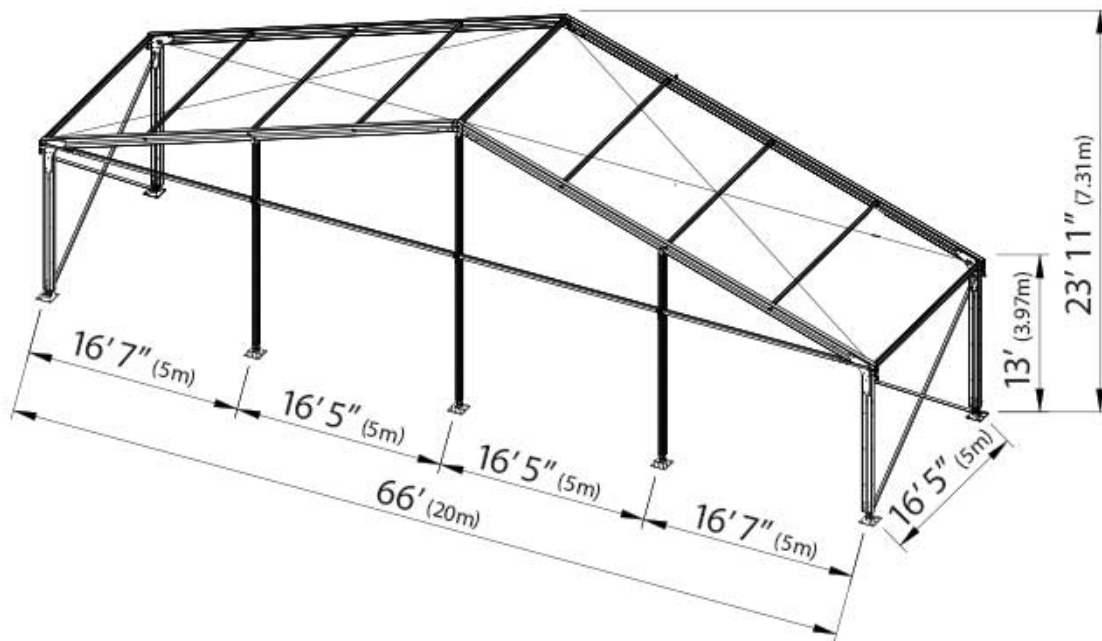
66' GABLE SPAN
