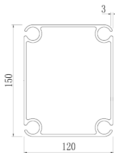
2. Gable Upright
