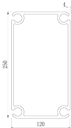
1. Main Profile
