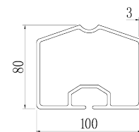
5. Gable Eave Rail
