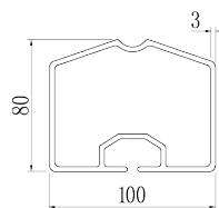
3. Eave Purlin
